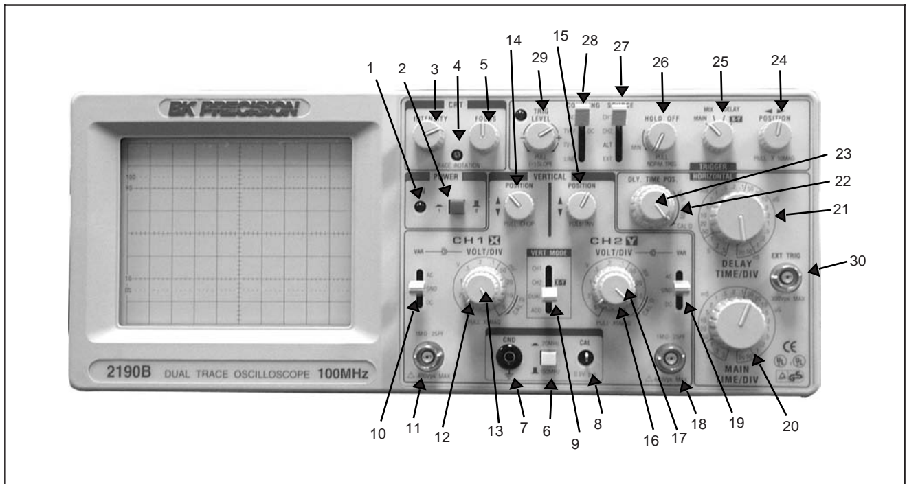
Fig. 1. Model 2190A Controls and Indicators.
