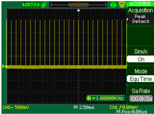
Figure 41 - Peak Detect
