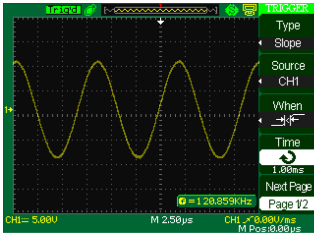
Figure 35 - Slope Trigger Menu
