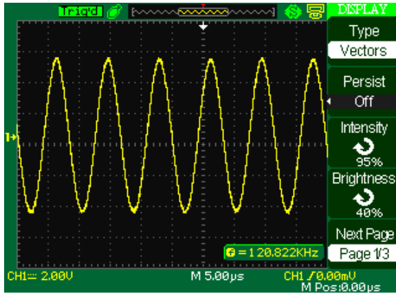
Figure 46 - Display Menu Screen
