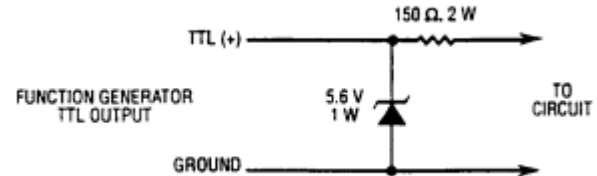
Figure 7. Circuit for Protection of TTL Output.
