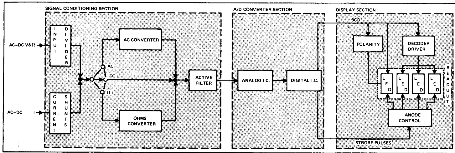
Figure 3-1. BLOCK DIAGRAM
