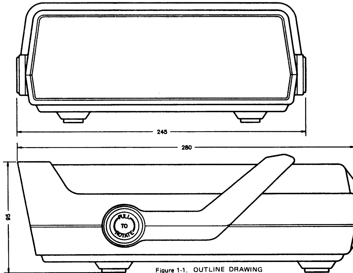
Figure 1-1. OUTLINE DRAWING
