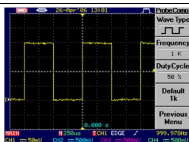
Fig. 1b Digital Storage Oscilloscope
