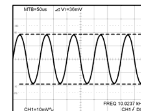
Figure 5-14: Cursor Measurement
