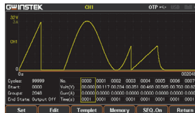
Output Waveform of the GPP-X323 Series
