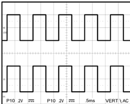
Figure 5-3 Function Check
