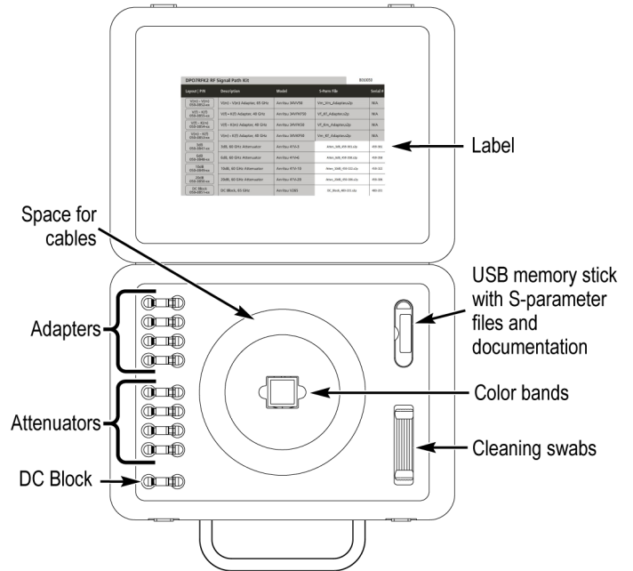
DPO7RFK2-Extended 1.85 mm characterized attenuator/adapter kit.
