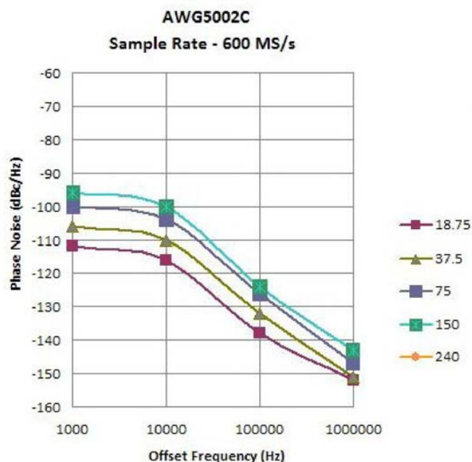
AWG5002C phase noise (typical).
