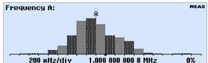
Histogram Plot.
